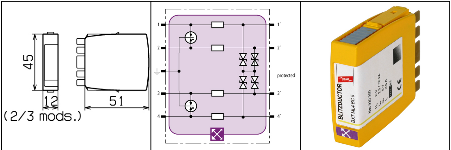
Dimension drawing BXT ML4 BC
