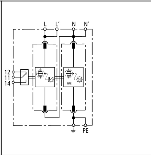
Basic circuit diagram DV M TT 2P 255 FM
