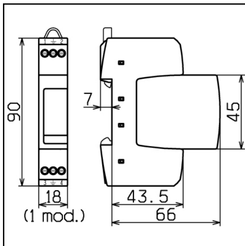
Dimension drawing DR M 2P ... FM
